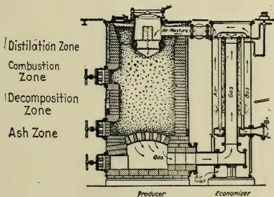
FIG. 95.—Loomis-Pettibone Suction Gas-Producer, Type 2.
